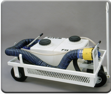
Lavatory Service Cart High durability, low maintenance
