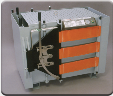
Aviation Tire Cage Only industry tested cage
