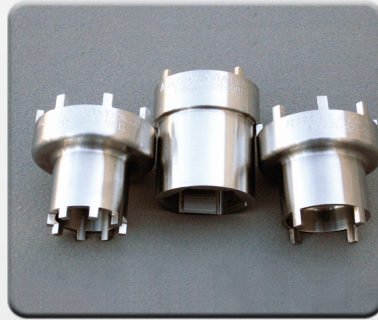
Falcon Spanner Sockets Dual sided 2 in 1 design
