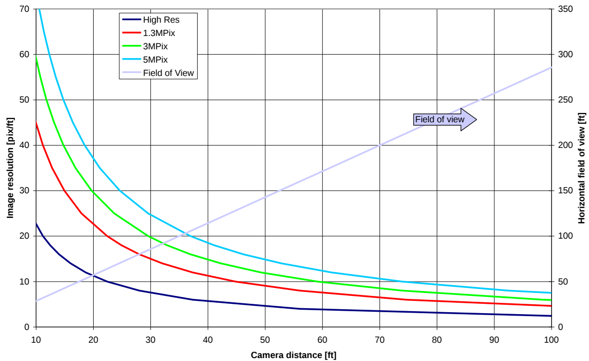
SY125 camera distance vs. image resolution and HFOV
