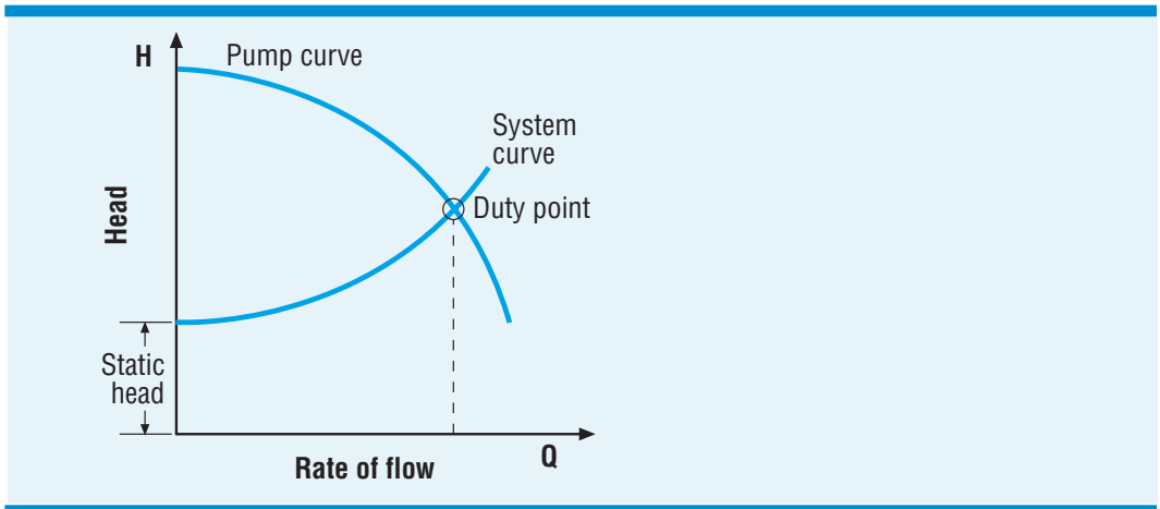
Figure 1. The duty point is the intersection between the pump and system curves
