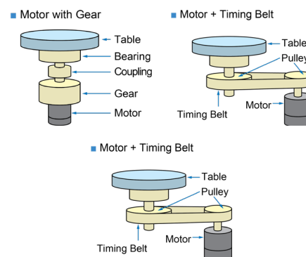
Figure 7: Mechanical designs
