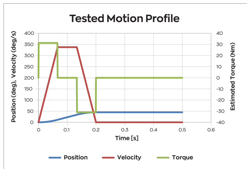
Figure 2: Tested motion profile
