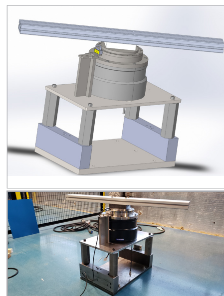
Figure 4: Direct drive motor setup
