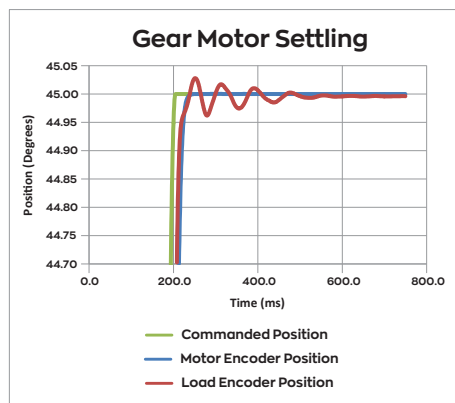
Figure 5: Gear motor oscillation at load
