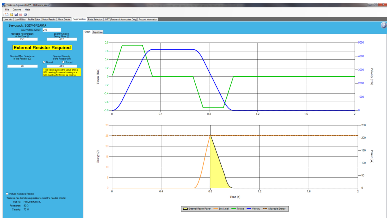
Figure 3: Calculations may show that an external regeneration resistor is required when using the Yaskawa SigmaSelect servo sizing software.
