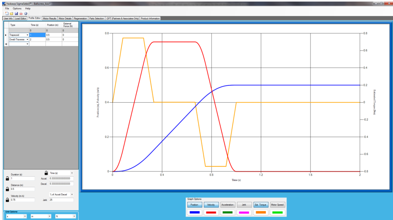
Figure 2: Speed/Torque curve from Yaskawa SigmaSelect servo sizing software plotting position (m) and velocity (m/s) on the vertical axis and time in seconds, horizontally.
