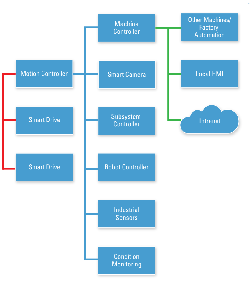
Decentralized Cooperative Machine Control System
