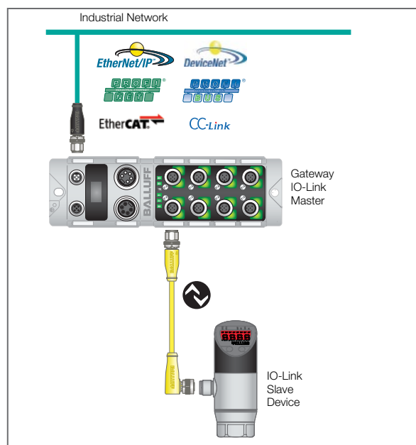
Figure 1: IO-Link architecture
