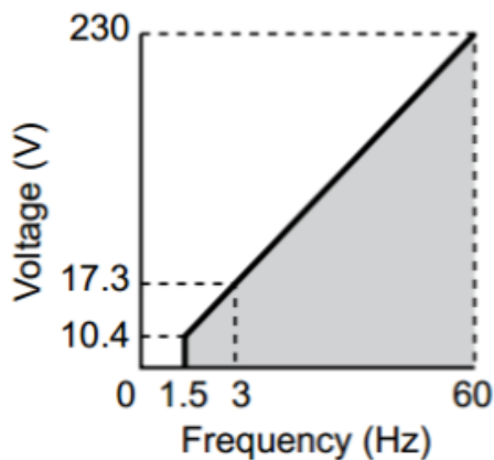
Constant torque V/f pattern
