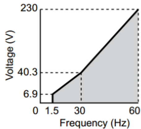
Variable torque V/f pattern
