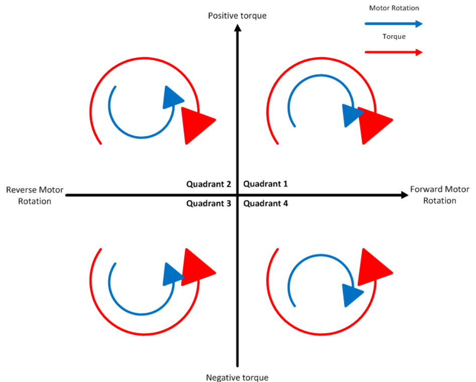
Figure 3: The Open loop vector control method allows for 4 quadrant torque limits
