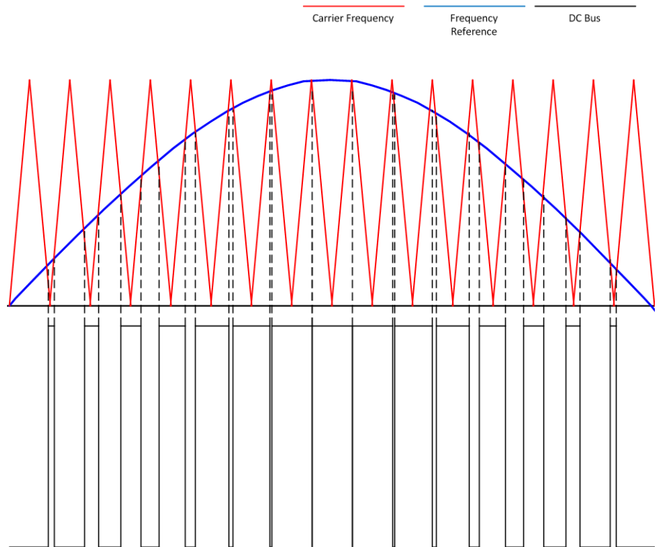
Figure 1: Pulse Width Modulation is used to Control an AC Motor
