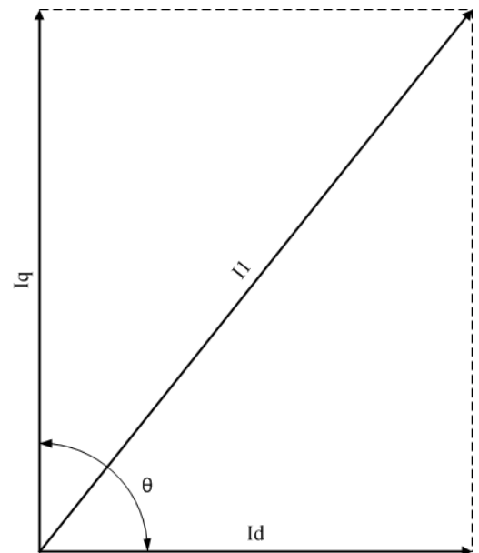
Figure 5: Vector control optimizes maximum torque per amp by keeping torque producing current ( I_q ) and magnetizing current ( I_d ) at 90°.
