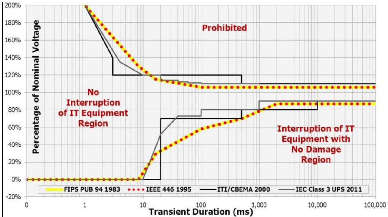
Figure 6: Historical perspective of IT equipment disturbance tolerance.
