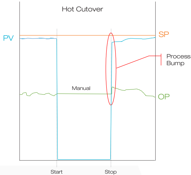
Process Trend on Cutover
