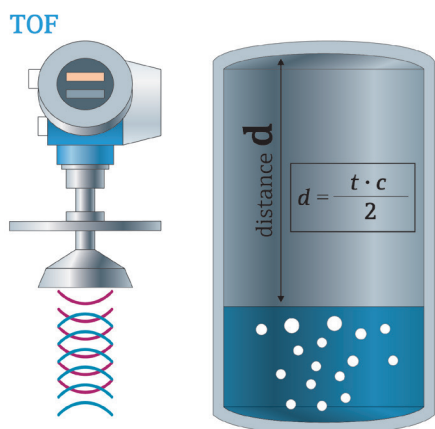
Figure 1: Time-of-flight radar calculates level based on the time it takes for a microwave pulse to travel to and return from the surface of the material being measured.
