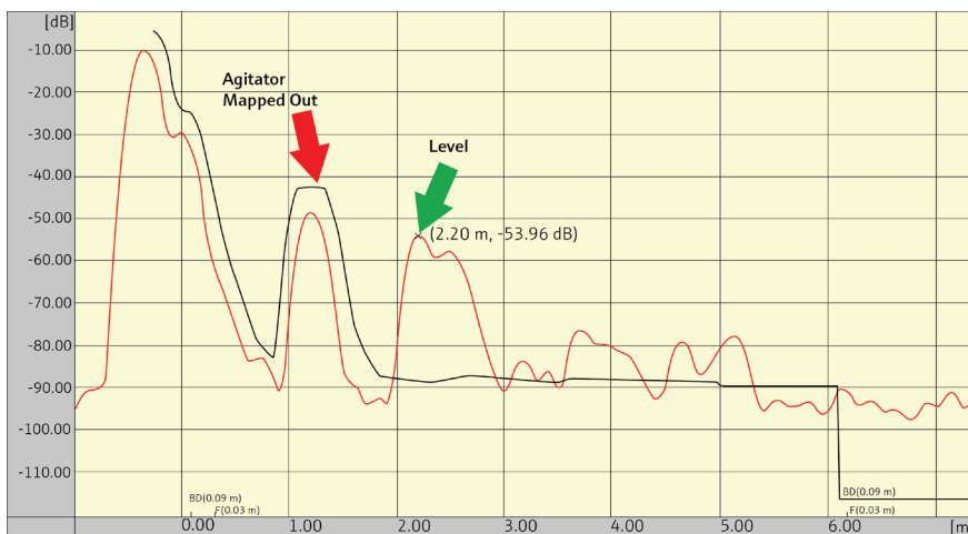
Figure 7: Envelope curve showing agitator signal mapped out.
