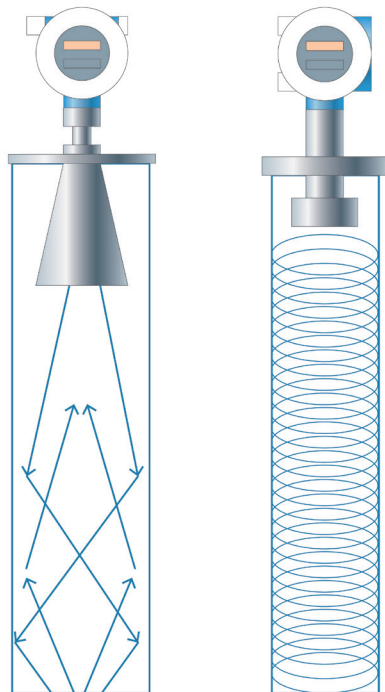
Figure 9: Radar signal from a horn antenna (left) in a stilling well does not follow a straight line. A planar antenna (right) is specially designed for stilling well applications.
