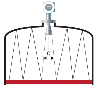
Figure 8: Mounting in the center of a tank can result in generating strong secondary reflections.
