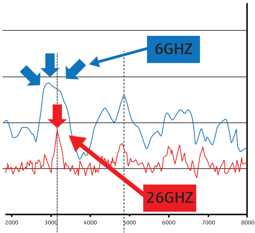
Figure 3: Comparison of 6 GHz and 26 GHz radar transmitters in the same application showing the sharp peak using 26 GHz to the rounded peak of a 6 GHz radar reflection.
