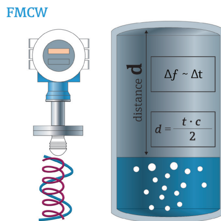
Figure 2: Frequency modulated continuous wave radar measures level based on the difference in frequency sent vs frequency being received.
