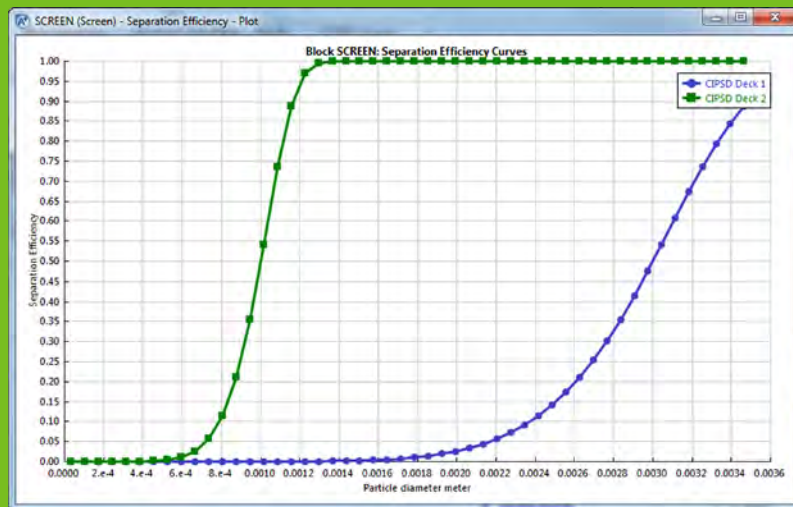
Figure 3: Example separation curves for a two-deck screen
