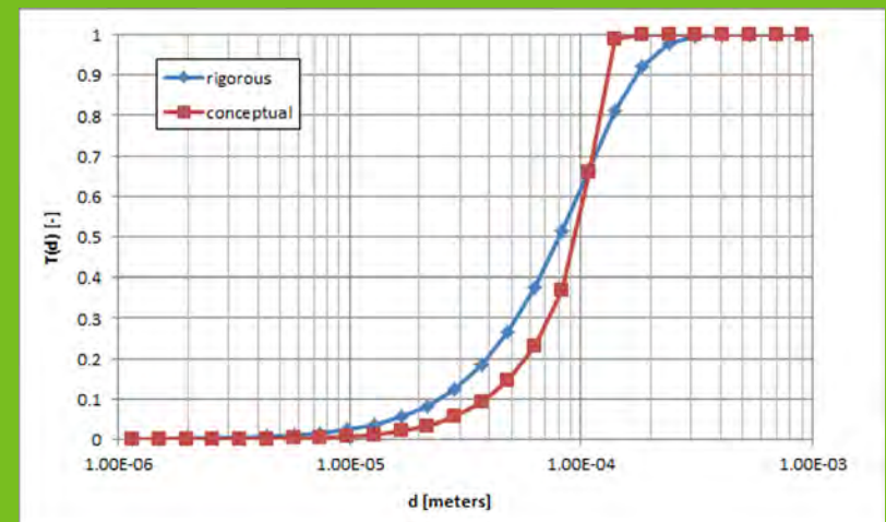
Figure 7: Comparison of the calculated separation efficiency curve for the conceptual centrifuge model (red curve) and the rigorous decenter model (blue curve)
