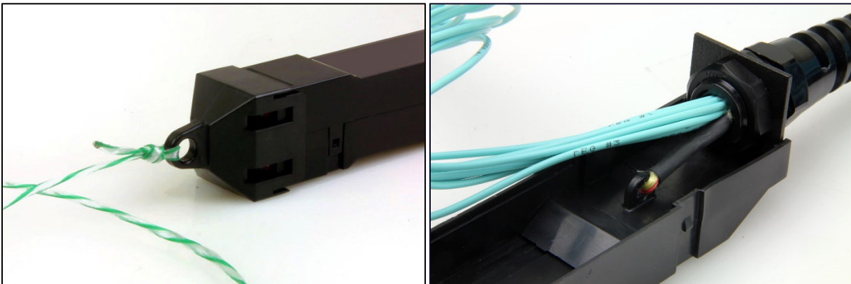
Figure 4: HDReadyLink™ trunks feature a patented HDReadyPull™ snap-on pulling cap and integrated strain relief that places the force on the strength members within the cable rather than the fibers
