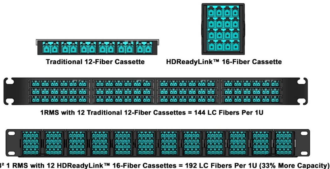
Figure 5: The square cassette design of the HDReadyLink™ trunks supports 16 LC fibers for 33% more capacity in 1U compared to traditional flat cassettes
