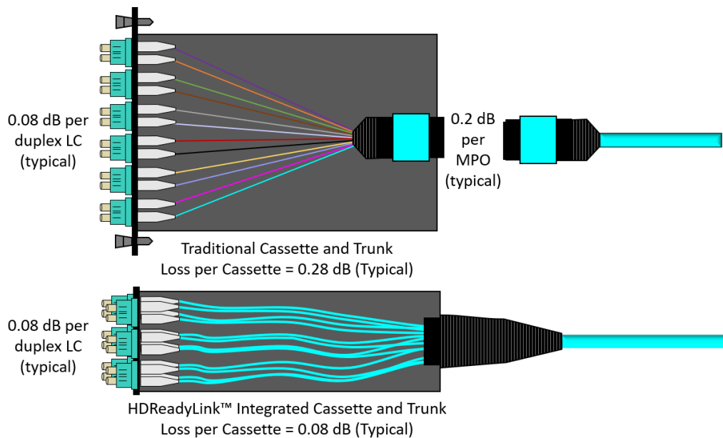
Figure 3: HDReadyLink™ integrated cassettes and trunks eliminate the rear MPO connection and associated loss
