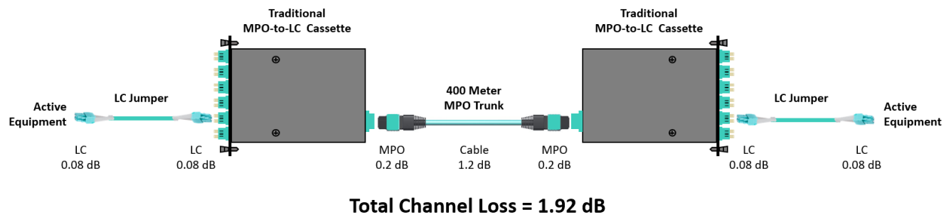
Figure 2: Channel loss for a 400m OM4 multimode fiber link using traditional cassettes
