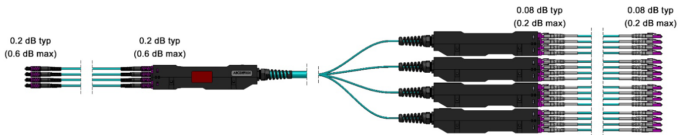
Figure 7: Test 2 utilized a 95-meter 10X4 aggregation channel with a total of 2 LC connections and 2 MPO connections
