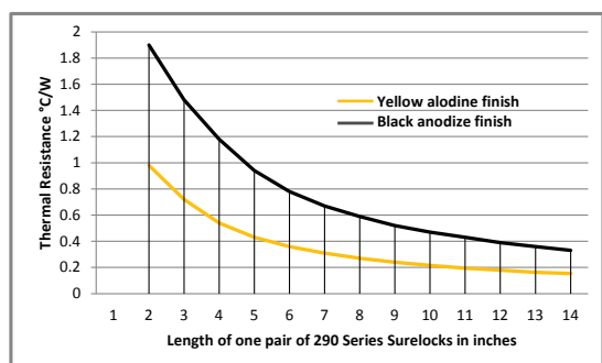
SureLock 290 Series – Thermal Resistance
