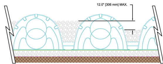
EVEN BACKFILL - CORRECT INSTALLATION
