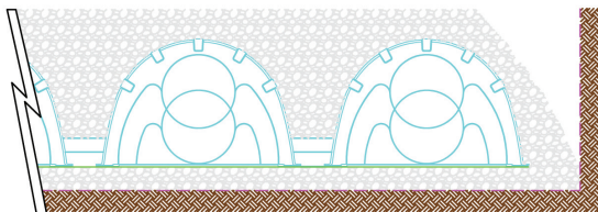
UNEVEN BACKFILL - INCORRECT INSTALLATION
